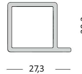
Code 862A Aluminium Profile
