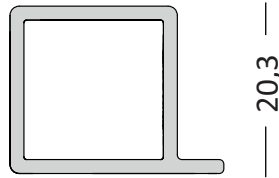
Code 862A Aluminium Profile
